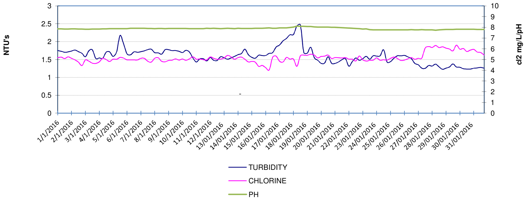
January, 2016 - Turbidity Chlorine & pH online monitoring-
