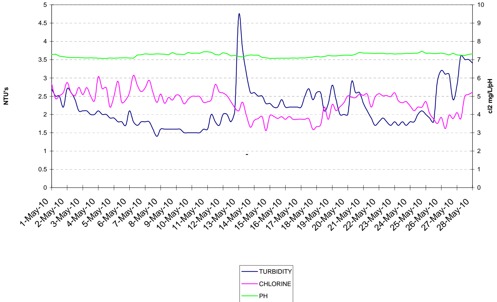
May, 2010 - Turbidity Chlor5ine & pH online monitoring-
